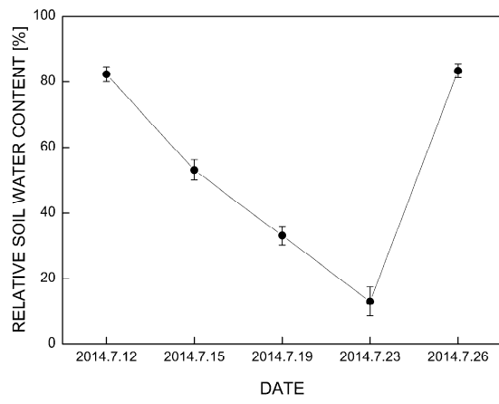
Fig. S1. The relative soil water content (RSWC, %) at the time of sample harvesting.
