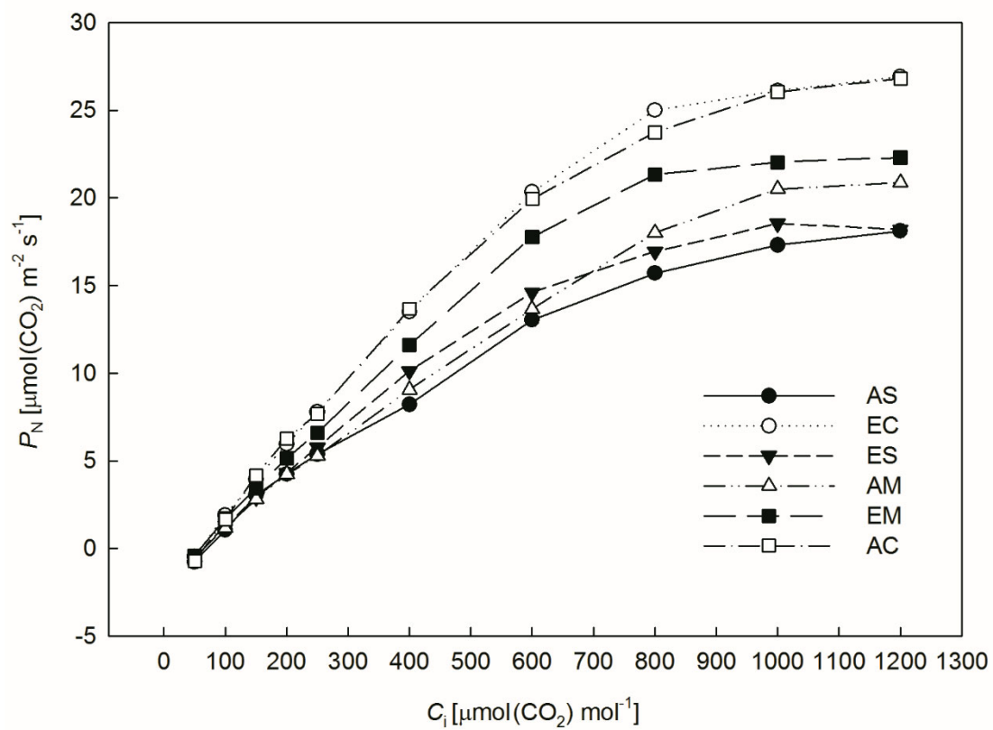
Fig. 5S. Effect of drought stress and elevated \text{CO}_2 on P_N/C_i curve.
