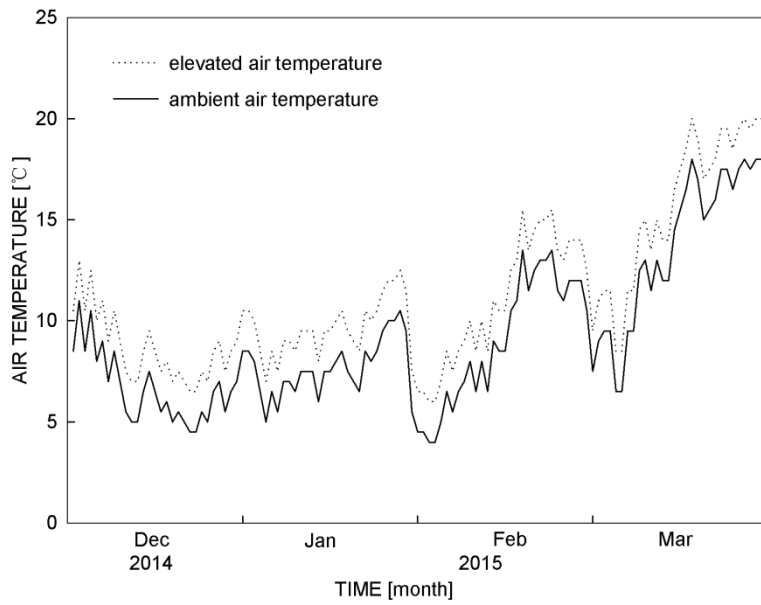
Fig. 1S. Winter air temperature (daily average) variation from December 2014 to March 2015. Broken and continuous lines indicate elevated and ambient air temperatures, respectively.
