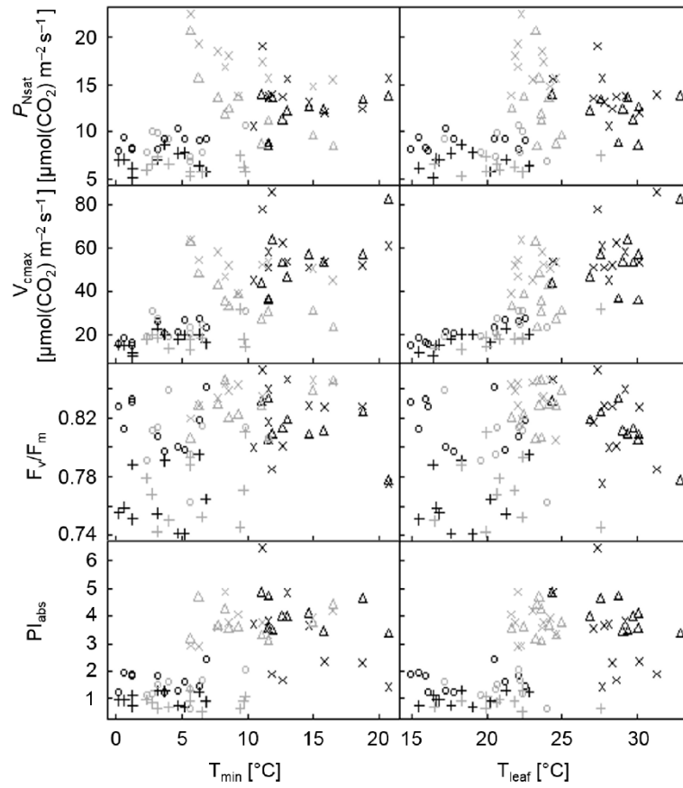
Fig. 1S. Parameters P_{Nsat} , V_{cmax} , F_v/F_m and PI_{abs} in relationship to minimum temperature of the night before the measurements on the left side of the panel and to leaf temperatures as measured during gas-exchange measurements in the right side. Indicated are the mean values per species, gradient and elevational band. Circles display A. foetida , triangles K. dipsacifolia , crosses represent M. perennis and squares T. pratense . Black symbols indicate Kramer gradient and dark grey symbols Kreuzeck.
