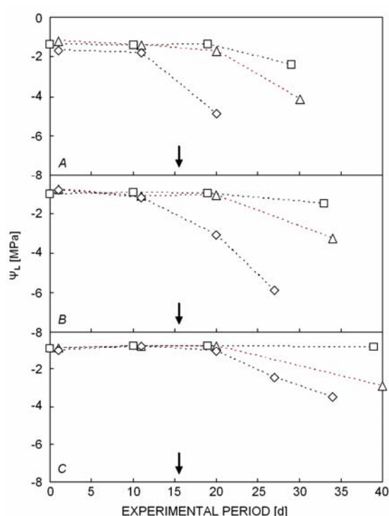
Fig. 3. Leaf water potential, \Psi_L during the experimental period in (A) Quercus cerris , (B) Q. frainetto , and (C) Q. ilex . Arrows indicate the change of relative humidity from 45 to 35 %. \diamond – set A; \square – set B; \triangle – set C.
