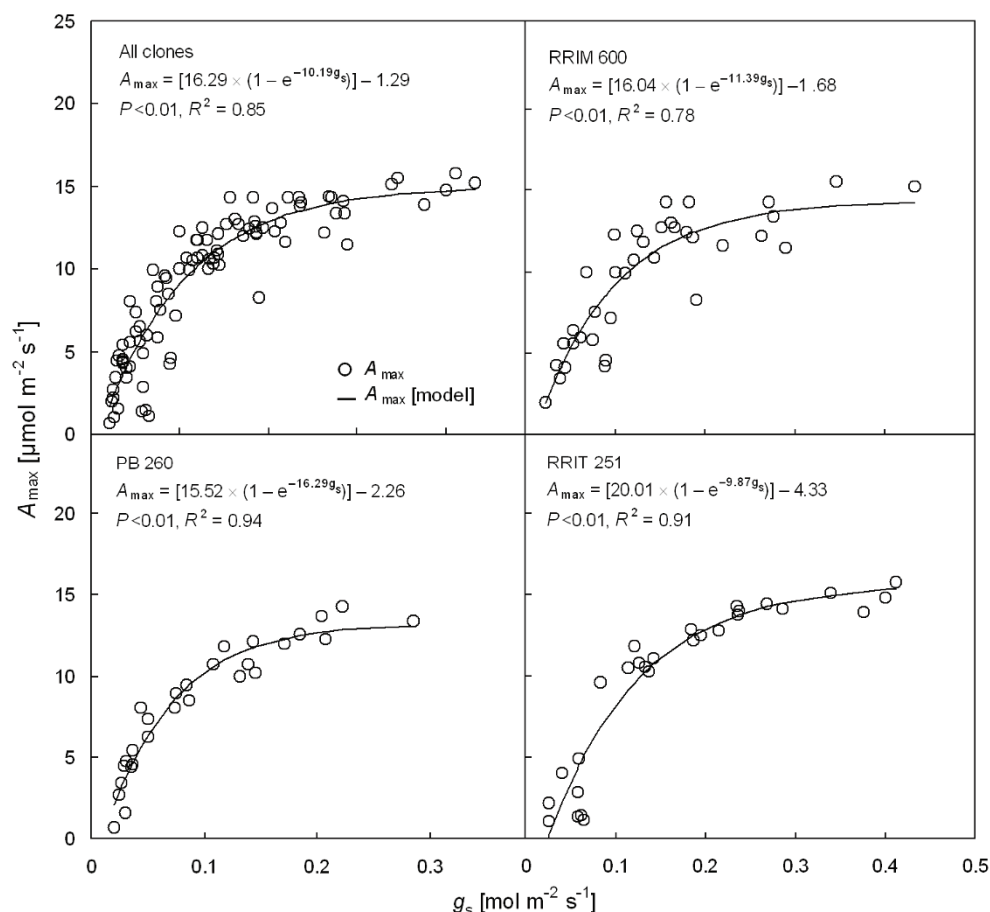
Fig. 5. Relationship between stomatal conductance ( g_s ) and light-saturated CO 2 assimilation rate ( A_{\max} ) of 2-year-old rubber trees. Dots represent observed data and the line represents an asymptotic function fitted to the observations. All clones pooled together ( top left ), clone RRIM 600 ( top right ), clone PB 260 ( bottom left ) and clone RRIT 251 ( bottom right ).
