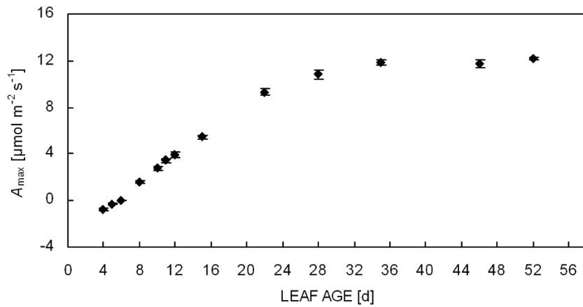
Fig. 2. Mean maximum rate of light-saturated \text{CO}_2 assimilation ( A_{\text{max}} ) as a function of leaf age of 2-month-old potted rubber, clone RRIM 600. Each value represents the average \pm SE ( n = 6 ).
