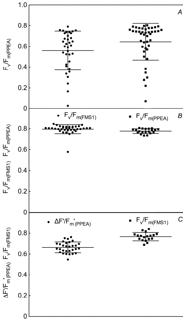
Fig. 2. Vertical scatter plot of maximum [ A , B (left and right), C (right)] or effective [ C (left)] quantum yield of PSII photochemistry measured on (i) dark-adapted leaves using the black clip/ Pocket PEA fluorometer [ F_v/F_m(\text{PPEA}) ; A (left and right), B (right)], (ii) light-adapted leaves using the black clip/ Pocket PEA fluorometer [ \Delta F'/F_m'(\text{PPEA}) ; C (left)], or (iii) dark-adapted leaves using the white clip/ FMSI fluorometer [ F_v/F_m(\text{FMSI}) ; B (left), C (right)]. A : Clipped-only tomato (left: 16 th June at 10:30 h; n = 35 ) or pepper (right: 9 th July at 11:00 h; n = 43 ) leaves. B : Clipped-only (left: pooled data from 11 th August at 09:40 and 10:35; n = 36 ) or clipped and shrouded (right: 11 th August at 11:30 h; n = 20 ) pepper leaves. C : Clipped-only tomato leaves measured on 9 th August at 10:00 h (left: n = 30 ) or 12:30 h (right: n = 18 ). The longer and the two shorter horizontal lines respectively indicate mean and SD of the data set. See text for data of global radiation ( R_g ).
