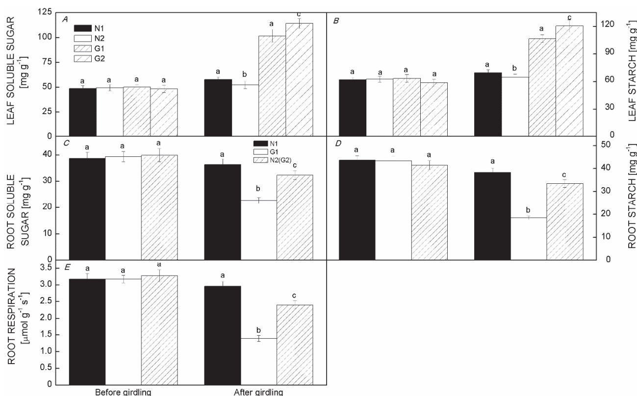
Fig. 2. Soluble sugar, starch, and root respiration of Alhagi sparsifolia under N1, N2, G1, and G2 treatment. A: leaf soluble sugar content, B: leaf starch content, C: root soluble sugar content, D: root starch content, E: root respiration of Alhagi sparsifolia before and after girdling. Different letters indicate significant difference ( p < 0.05 ). The data represent means of five biological replicates \pm SD. N1 – nongirdling with one branch left; G1 – girdling with one branch left; N2 – nongirdling with two branches left; G2 – girdling with two branches left.
