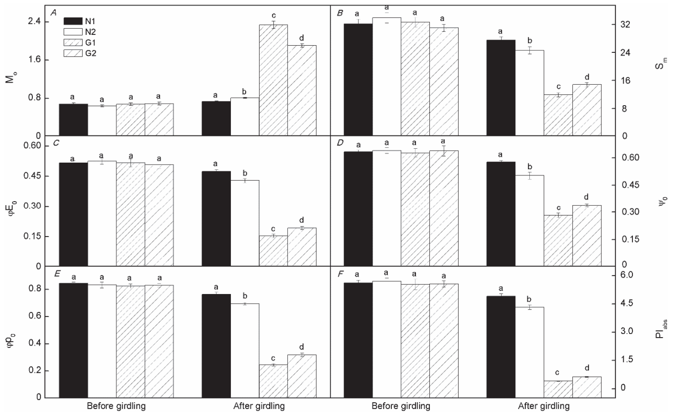
Fig. 7. M_0 , S_m , \phi_{E_0} , \psi_0 , \phi_{P_0} , and PI_{abs} of Alhagi sparsifolia under N1, N2, G1, and G2 treatment. M_0 – approximated initial slope of the fluorescence transient; S_m – normalised total complementary area above the OJIP transients (reflecting single-turnover Q_A reduction events); \phi_{E_0} – quantum yield for electron transport (at t = 0 ); \psi_0 – probability that a trapped exciton moves an electron into the electron transport chain beyond Q_A^- (at t = 0 ); \phi_{P_0} – maximum quantum yield for primary photochemistry (at t = 0 ); PI_{abs} – performance index on absorption basis. Different letters indicate a significant difference ( p < 0.05 ). The data represent means of five biological replicates \pm SD. N1 – nongirdling with one branch left; G1 – girdling with one branch left; N2 – nongirdling with two branches left; G2 – girdling with two branches left.
