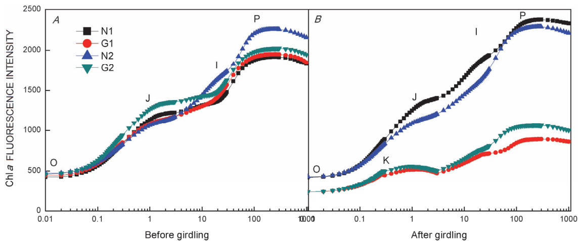
Fig. 8. OJIP chlorophyll (Chl) a fluorescence transient curves (log time scale) in Alhagi sparsifolia in the four treatments (N1, G1, N2, and G2) before (A) and after (B) girdling. N1 – nongirdling with one branch left; G1 – girdling with one branch left; N2 – nongirdling with two branches left; G2 – girdling with two branches left.
