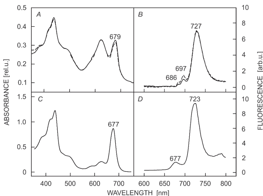
Fig. 1. Room temperature absorption (A,C) and 77 K low temperature chlorophyll fluorescence (B,D) spectra of the Synechocystis 6803 cells (A,B) of wild type (solid line) and mutant expressing PsaF-YFP (WT-YFP; dashed line), and of the preparation isolated using GFP-Trap® from the WT-YFP mutant (C,D). The numbers designate absorption and emission maxima in nm.
