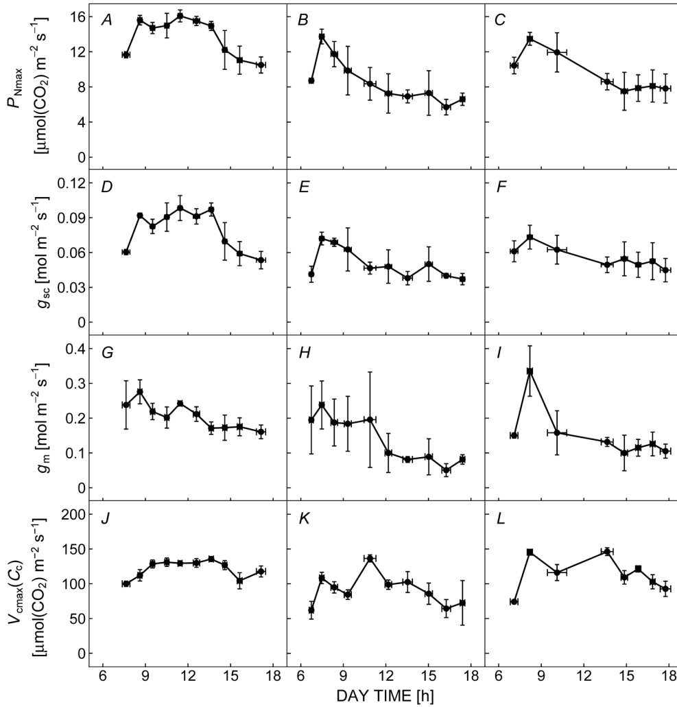
Fig. 4. Diurnal changes in light-saturated photosynthetic rate ( P_{Nmax} ) (A–C), stomatal conductance to CO_2 ( g_{sc} ) (D–F), mesophyll conductance ( g_m ) (G–I), and maximum carboxylation rate based on the CO_2 concentration at the carboxylation site [ V_{cmax}(C_c) ] (J–L). The respective rows indicate the day when gas-exchange measurements were conducted ( i.e. , A, D, G, J: 22 May; B, E, H, K: 23 May; C, F, I, L: 30 May). The measurements were conducted from 6:30 to 18:00 h (Japan standard time). Means \pm SE ( n = about 3) are shown.
