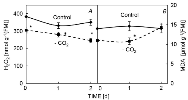
Fig. 4. The content of H 2 O 2 (A) and malondialdehyde (MDA) (B) in the 2 nd leaves immediately after opening the incubation chamber at low CO 2 concentration and during the next 2 d (–CO 2 ) in comparison with plants growing at a natural CO 2 concentration (Control). Data are means ± SE. Values between curves ‘Control’ and ‘–CO 2 ’ marked with an asterisk differ at the p < 0.05 level.
