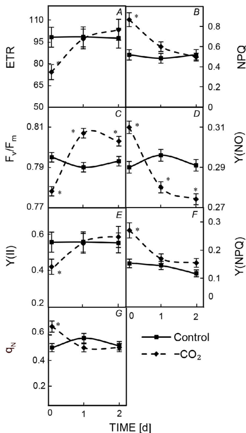
Fig. 3. Fluorescence parameters of 2 nd leaf immediately after opening the incubation chamber with plants at a low concentration of CO 2 and during the next 2 d (–CO 2 ) in comparison with plants growing at a natural concentration of CO 2 (Control). Data are means ± SE. Values between curves ‘Control’ and ‘–CO 2 ’ marked with an asterisk differ at the p < 0.05 level. Here, ETR – electron transport rate, F_v/F_m and Y_{(II)} – PSII maximal and effective quantum yields, respectively, q_N and NPQ – parameters of nonphotochemical quenching. Y_{(NO)} – non-light-induced nonphotochemical fluorescence quenching and Y_{(NPQ)} – light-induced nonphotochemical fluorescence quenching regulated.
